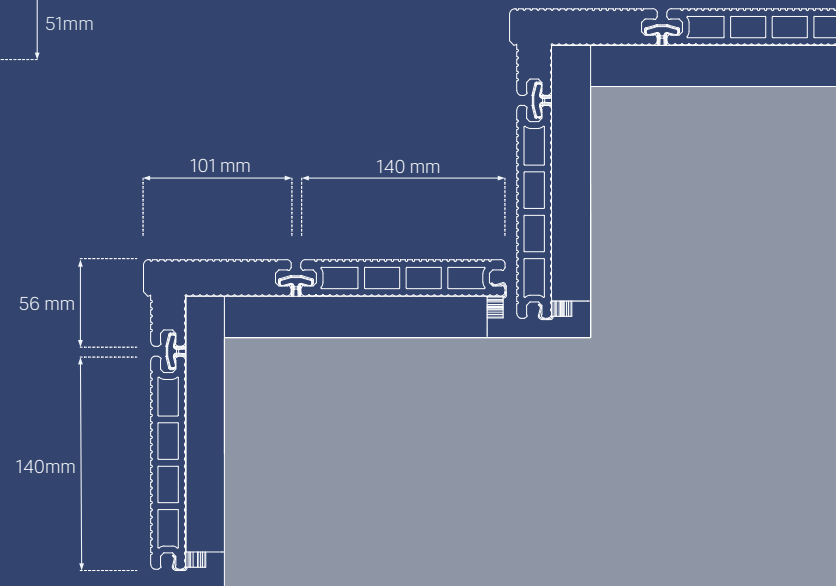
DEGRAU CDECK ESCALÓN CDECK
